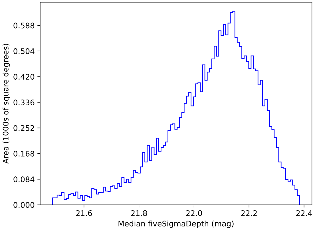
extra_ss_neo7_v3.4_10yrs Yr 1 y band: Median fiveSigmaDepth
