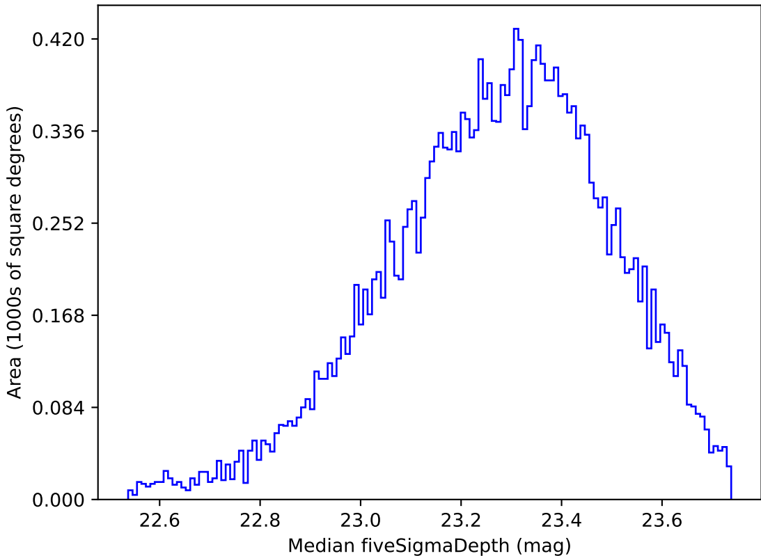
extra_ss_neo7_v3.4_10yrs Yr 1 u band: Median fiveSigmaDepth
