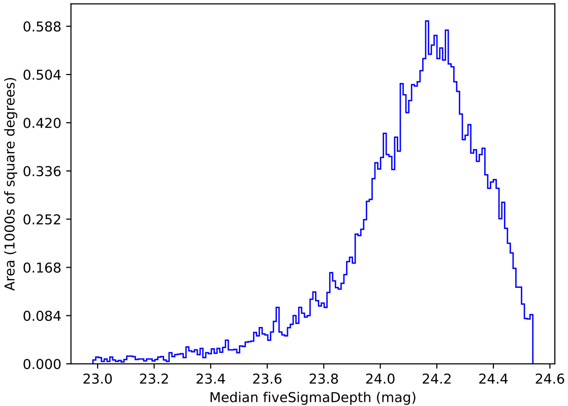
extra_ss_neo7_v3.4_10yrs Yr 1 r band: Median fiveSigmaDepth
