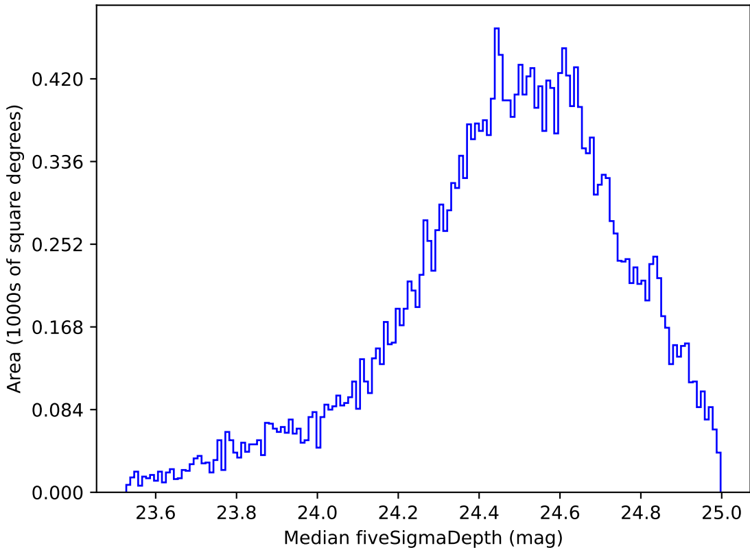
extra_ss_neo7_v3.4_10yrs Yr 1 g band: Median fiveSigmaDepth
