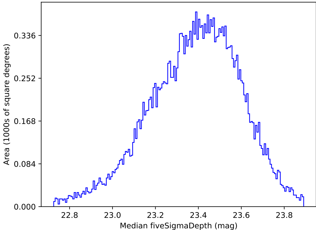
extra_ss_neo7_v3.4_10yrs Yr 1 all bands: Median fiveSigmaDepth
