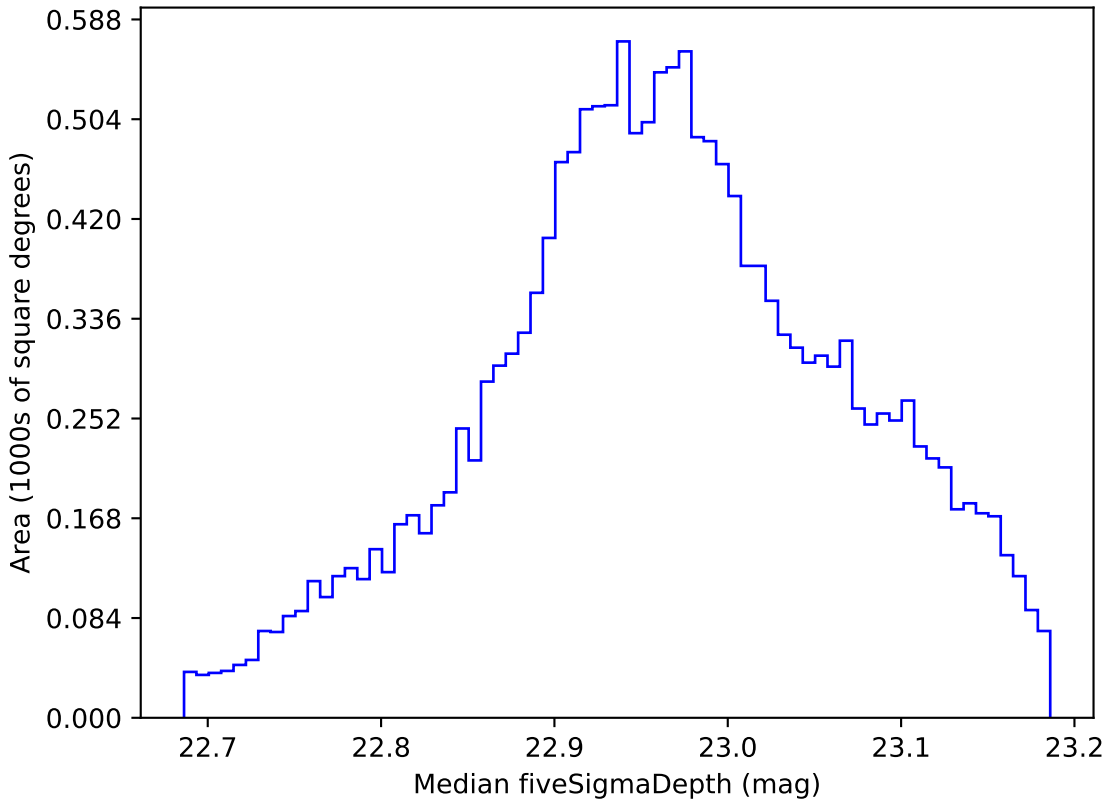
extra_ss_neo7_v3.4_10yrs WFD z band: Median fiveSigmaDepth
