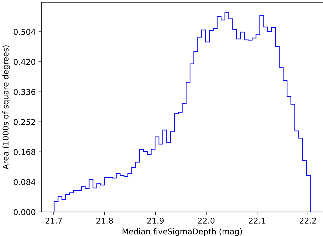
extra_ss_neo7_v3.4_10yrs WFD y band: Median fiveSigmaDepth
