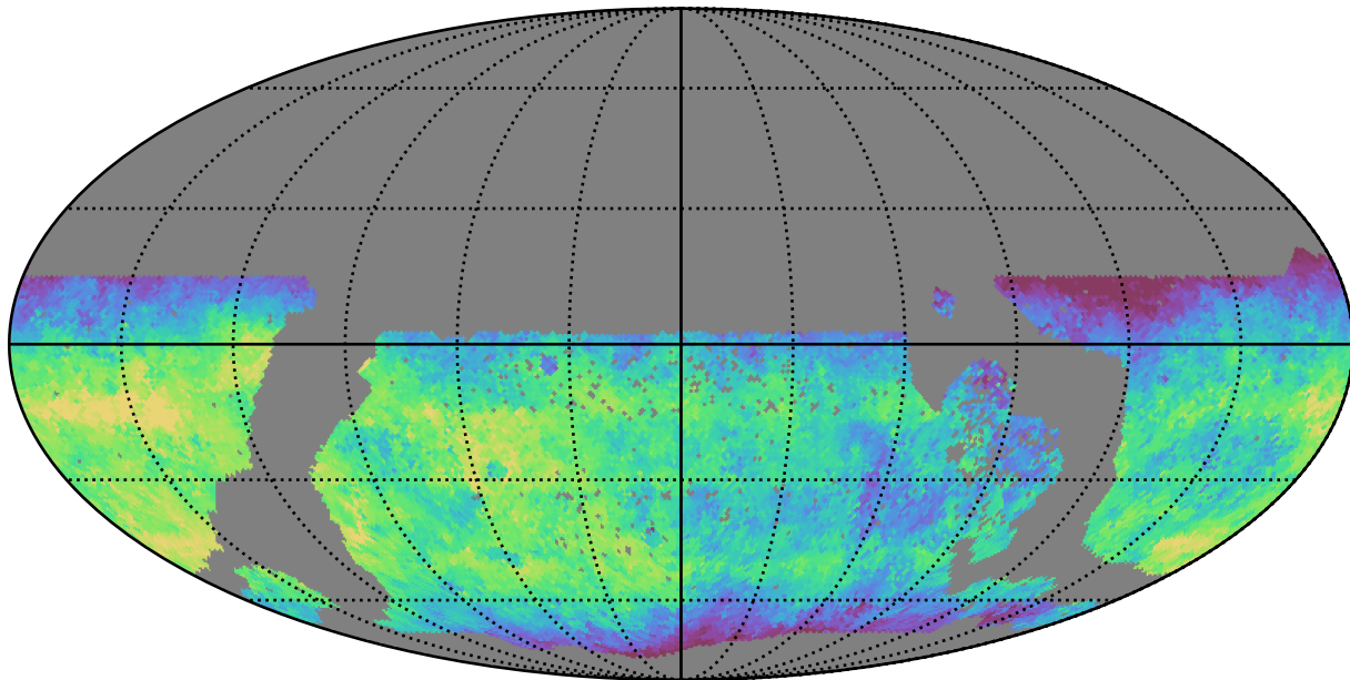
extra_ss_neo7_v3.4_10yrs WFD u band: Median fiveSigmaDepth
