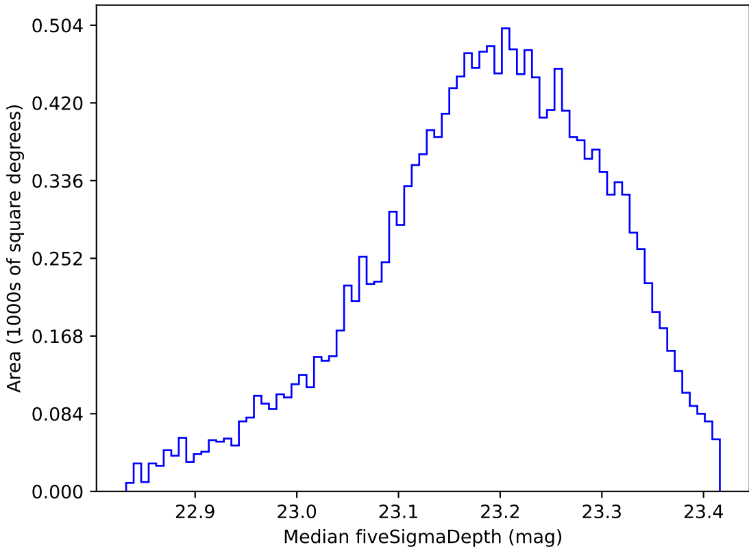
extra_ss_neo7_v3.4_10yrs WFD u band: Median fiveSigmaDepth
