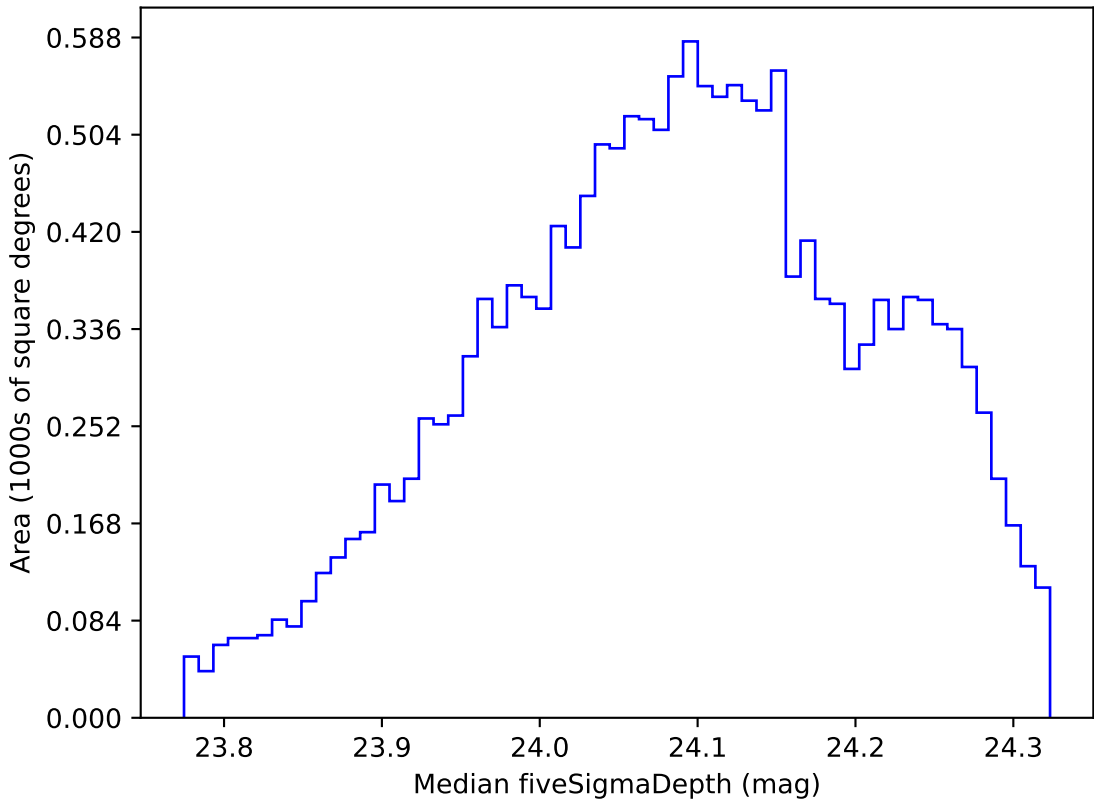
extra_ss_neo7_v3.4_10yrs WFD r band: Median fiveSigmaDepth
