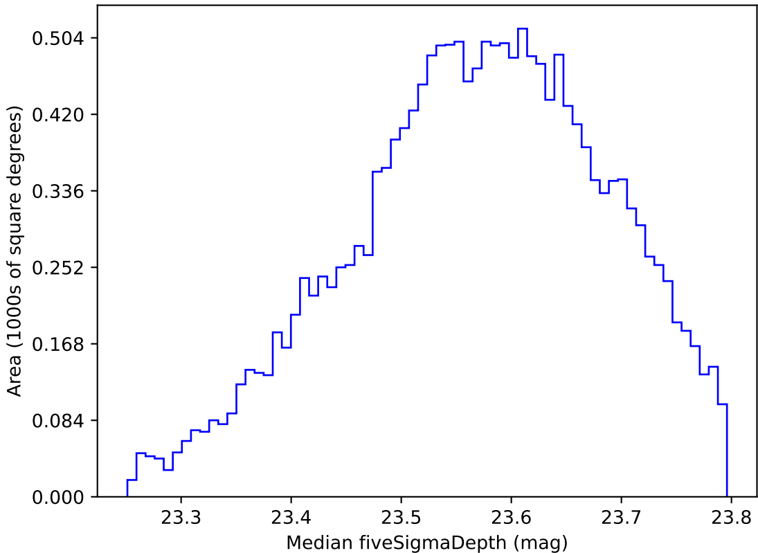
extra_ss_neo7_v3.4_10yrs WFD i band: Median fiveSigmaDepth
