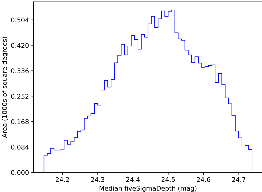
extra_ss_neo7_v3.4_10yrs WFD g band: Median fiveSigmaDepth
