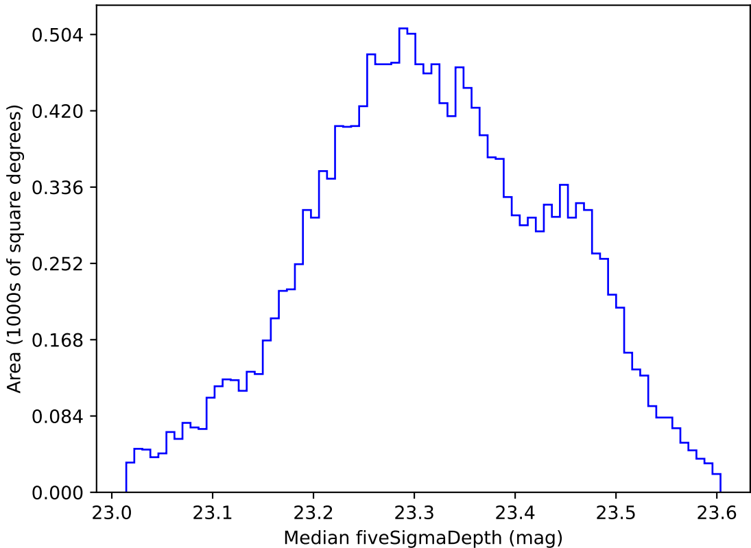
extra_ss_neo7_v3.4_10yrs WFD all bands: Median fiveSigmaDepth
