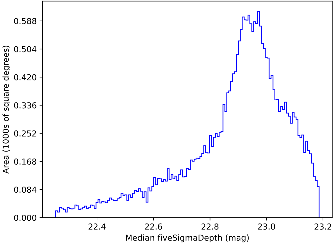
extra_ss_neo7_v3.4_10yrs All sky z band: Median fiveSigmaDepth
