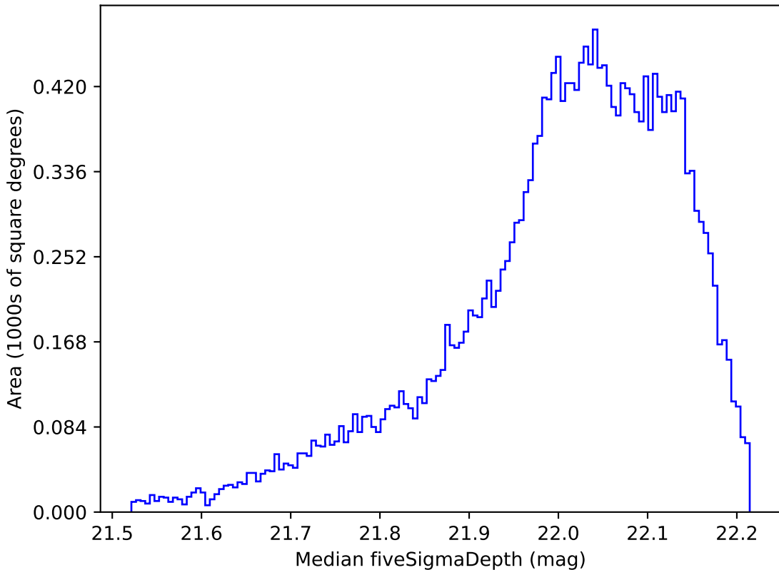
extra_ss_neo7_v3.4_10yrs All sky y band: Median fiveSigmaDepth
