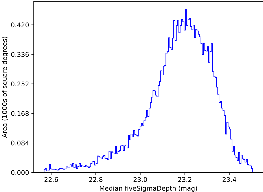
extra_ss_neo7_v3.4_10yrs All sky u band: Median fiveSigmaDepth
