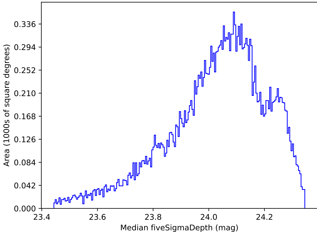
extra_ss_neo7_v3.4_10yrs All sky r band: Median fiveSigmaDepth
