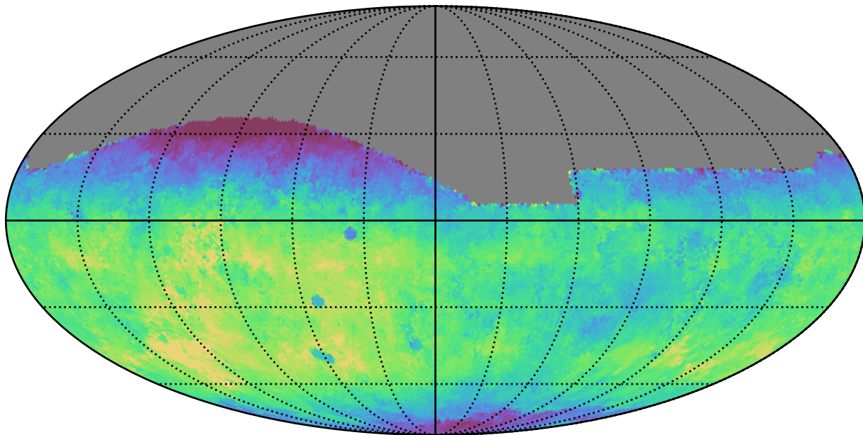
extra_ss_neo7_v3.4_10yrs All sky g band: Median fiveSigmaDepth
