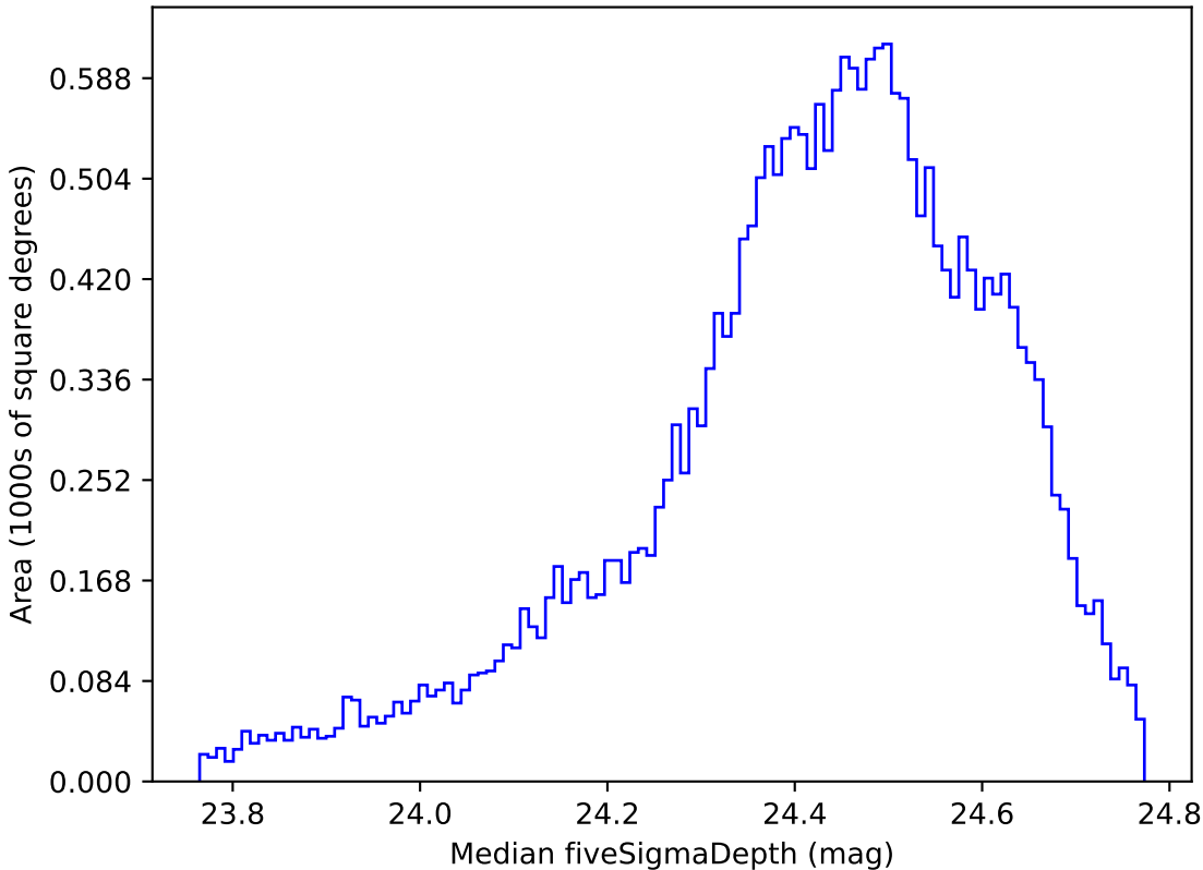
extra_ss_neo7_v3.4_10yrs All sky g band: Median fiveSigmaDepth
