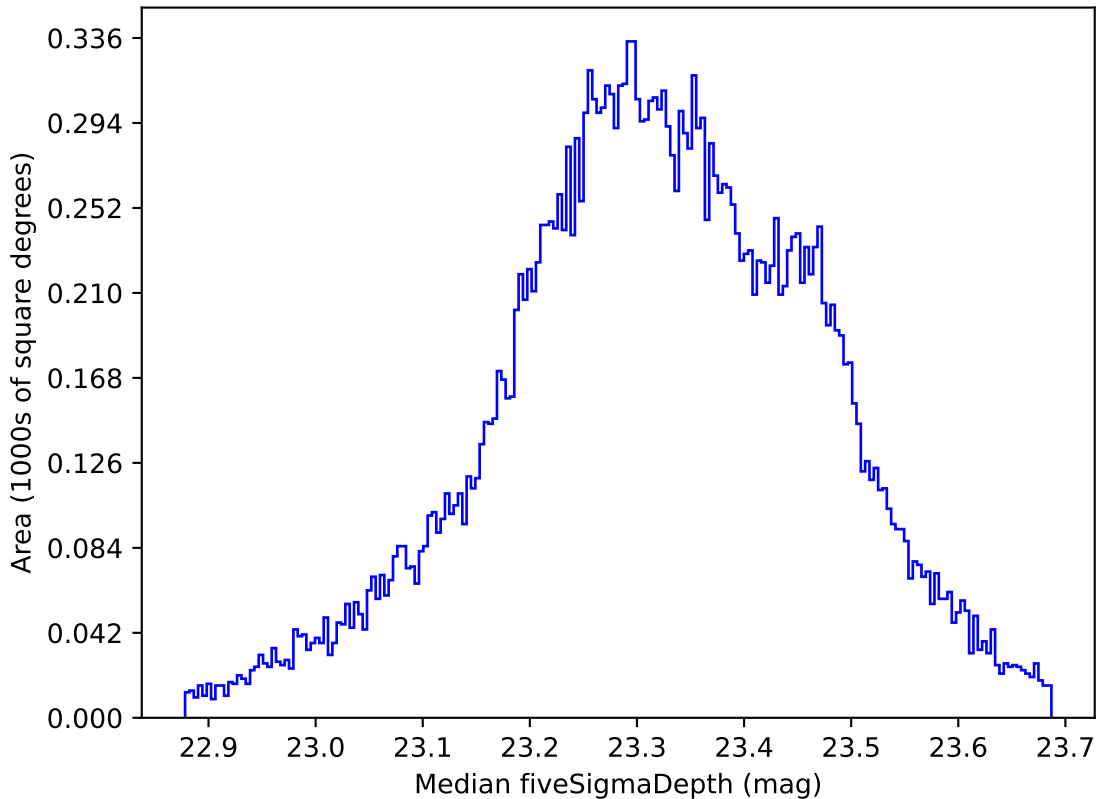
extra_ss_neo7_v3.4_10yrs All sky all bands: Median fiveSigmaDepth
