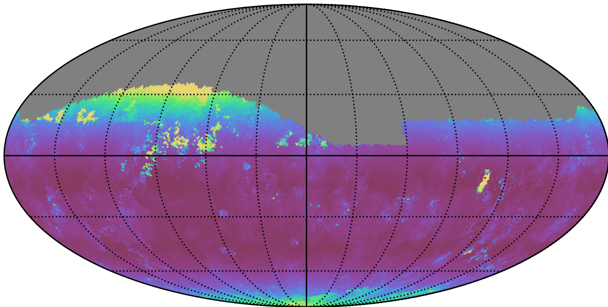
extra_ss_neo7_v3.4_10yrs Yr 1 z band: Median airmass
