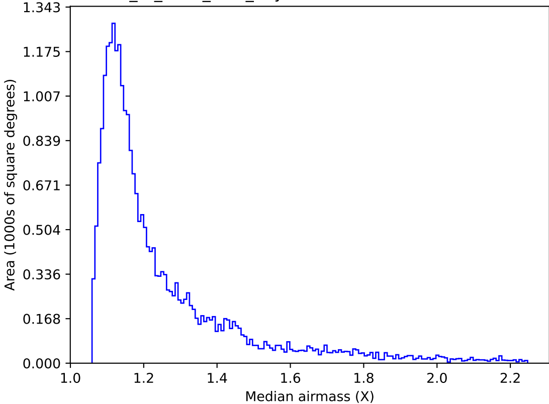
extra_ss_neo7_v3.4_10yrs Yr 1 z band: Median airmass
