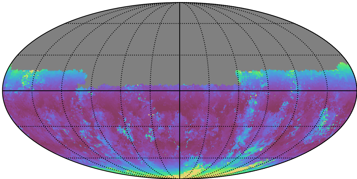
extra_ss_neo7_v3.4_10yrs Yr 1 u band: Median airmass
