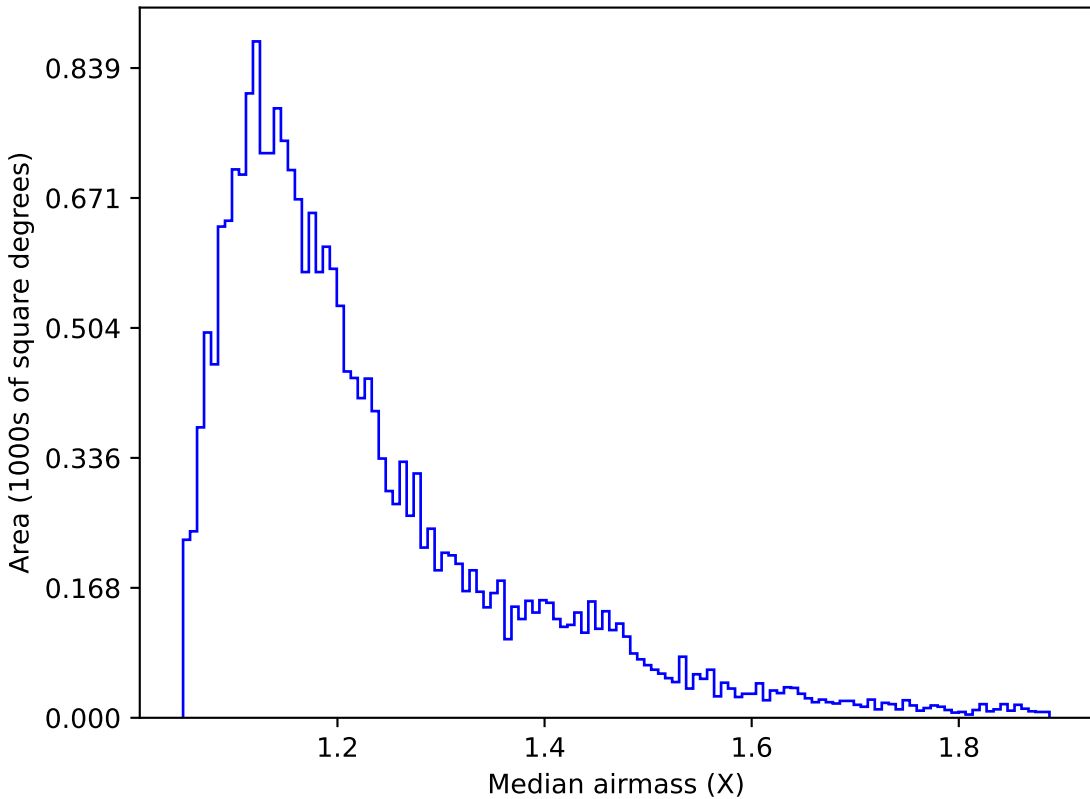
extra_ss_neo7_v3.4_10yrs Yr 1 u band: Median airmass
