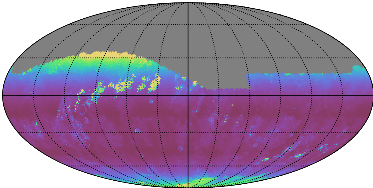
extra_ss_neo7_v3.4_10yrs Yr 1 r band: Median airmass
