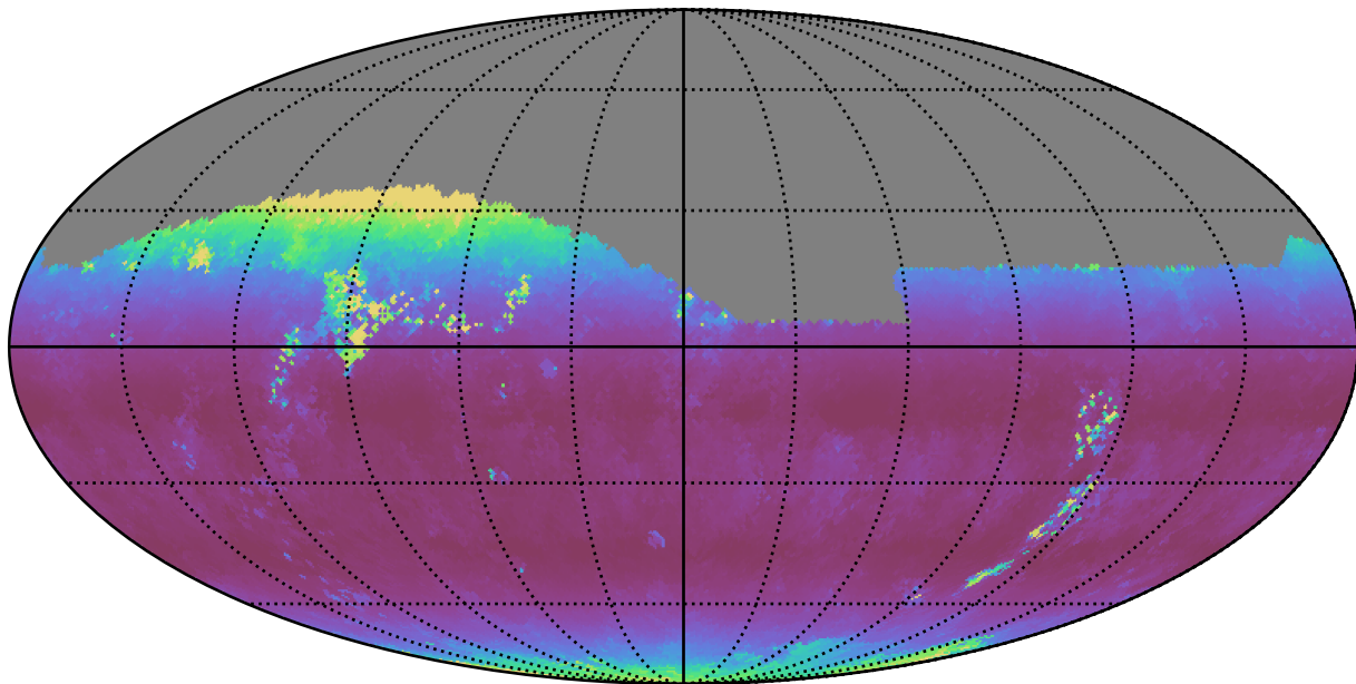
extra_ss_neo7_v3.4_10yrs Yr 1 i band: Median airmass
