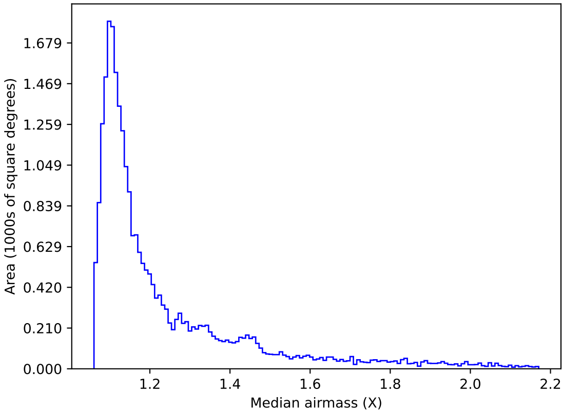
extra_ss_neo7_v3.4_10yrs Yr 1 i band: Median airmass
