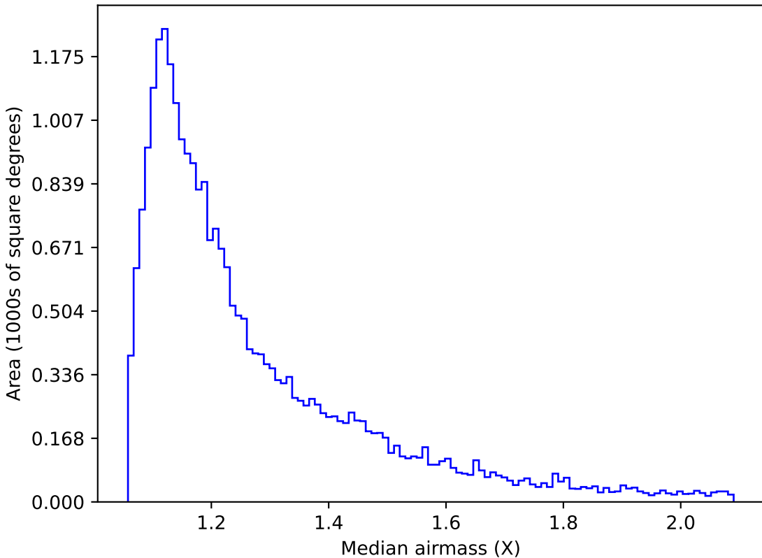
extra_ss_neo7_v3.4_10yrs Yr 1 g band: Median airmass
