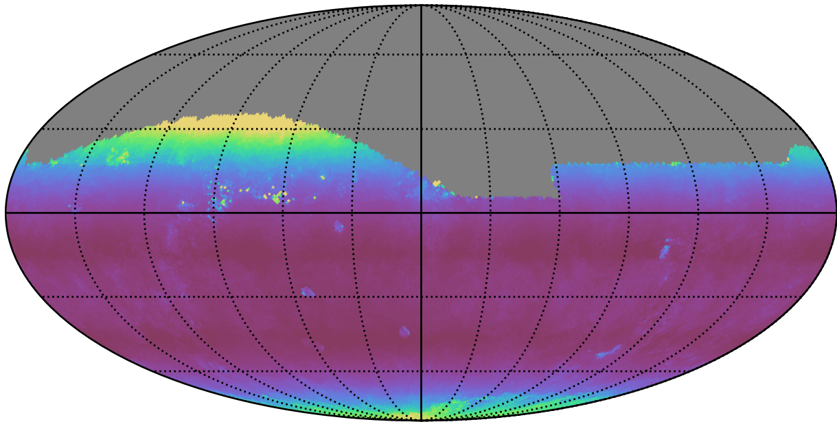
extra_ss_neo7_v3.4_10yrs Yr 1 all bands: Median airmass
