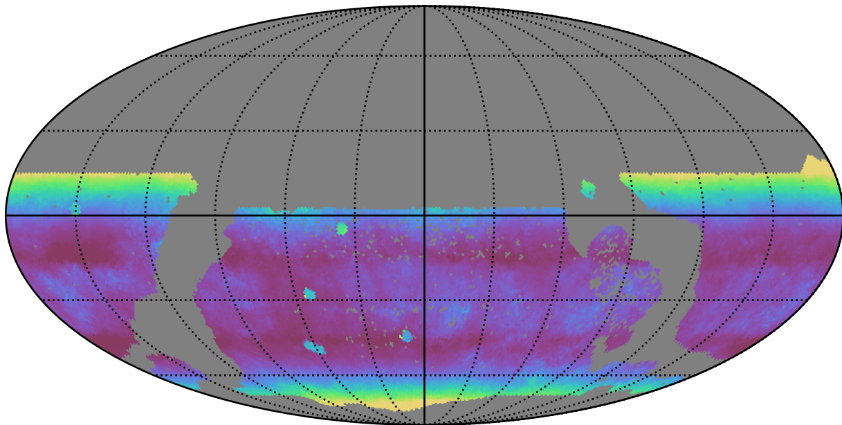
extra_ss_neo7_v3.4_10yrs WFD z band: Median airmass
