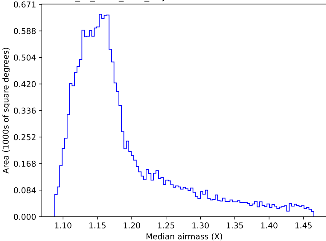
extra_ss_neo7_v3.4_10yrs WFD z band: Median airmass
