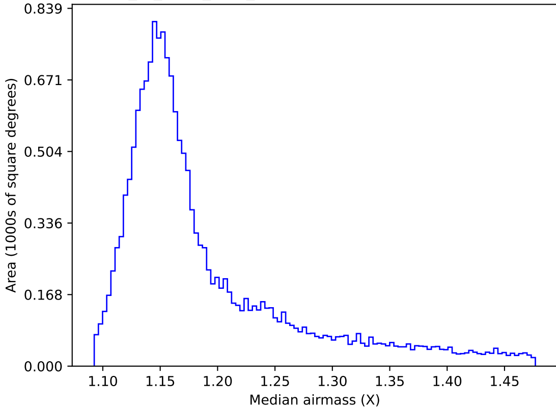
extra_ss_neo7_v3.4_10yrs WFD y band: Median airmass
