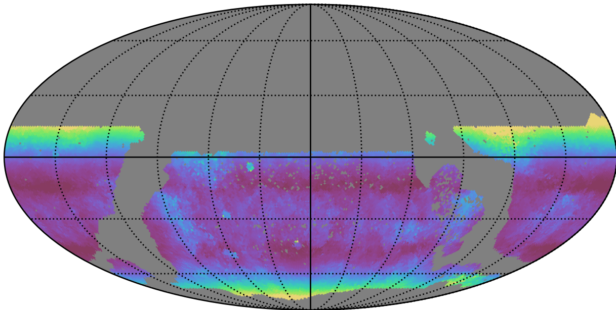
extra_ss_neo7_v3.4_10yrs WFD u band: Median airmass
