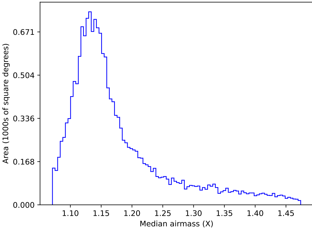
extra_ss_neo7_v3.4_10yrs WFD u band: Median airmass
