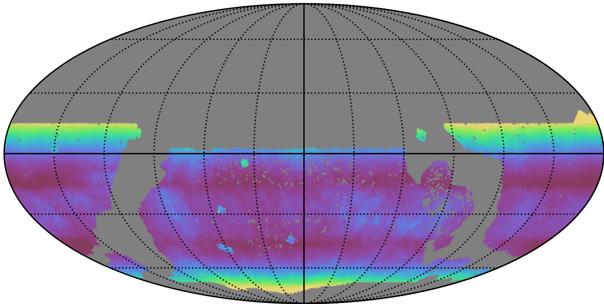
extra_ss_neo7_v3.4_10yrs WFD r band: Median airmass
