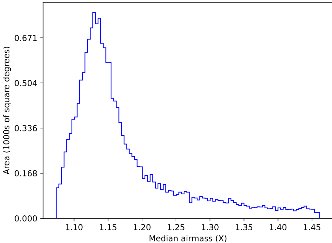
extra_ss_neo7_v3.4_10yrs WFD r band: Median airmass
