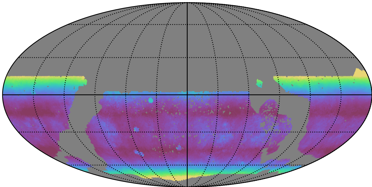
extra_ss_neo7_v3.4_10yrs WFD i band: Median airmass
