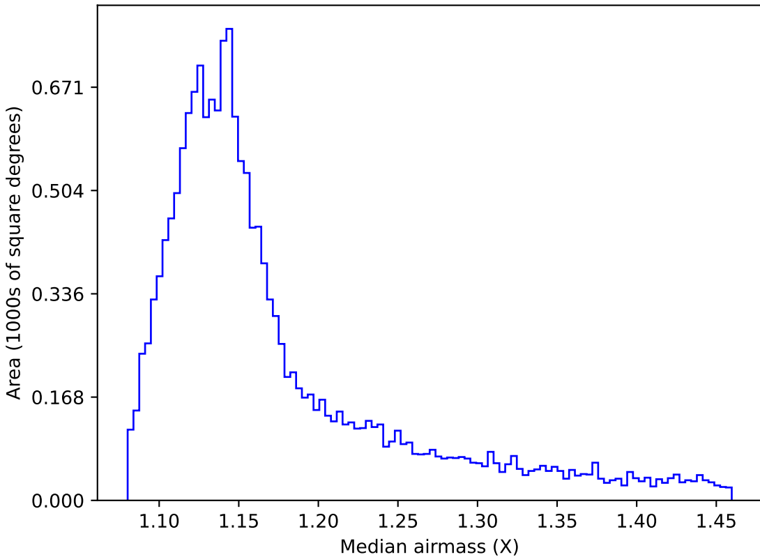
extra_ss_neo7_v3.4_10yrs WFD i band: Median airmass
