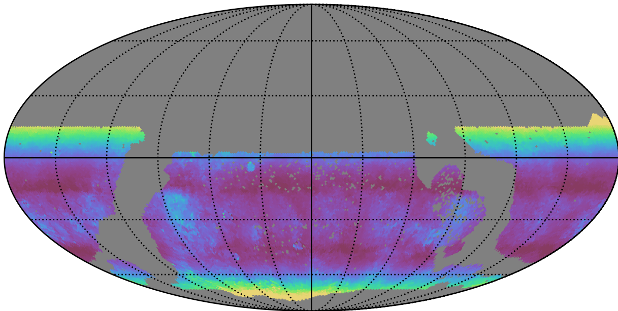
extra_ss_neo7_v3.4_10yrs WFD g band: Median airmass
