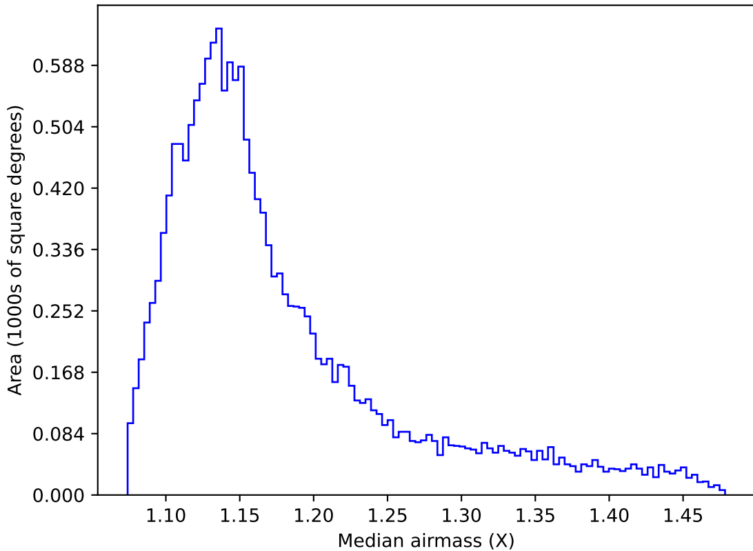
extra_ss_neo7_v3.4_10yrs WFD g band: Median airmass
