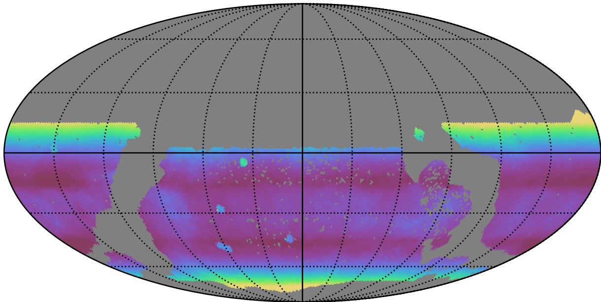
extra_ss_neo7_v3.4_10yrs WFD all bands: Median airmass
