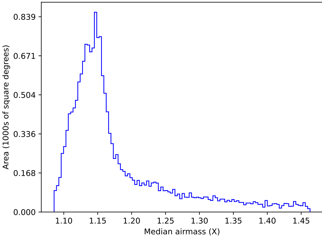
extra_ss_neo7_v3.4_10yrs WFD all bands: Median airmass
