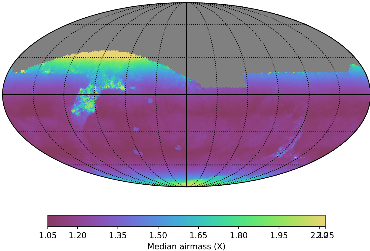
extra_ss_neo7_v3.4_10yrs All sky z band: Median airmass
