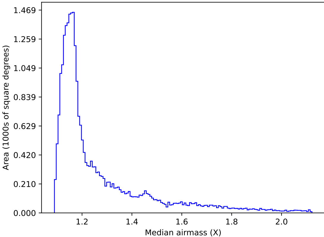
extra_ss_neo7_v3.4_10yrs All sky z band: Median airmass
