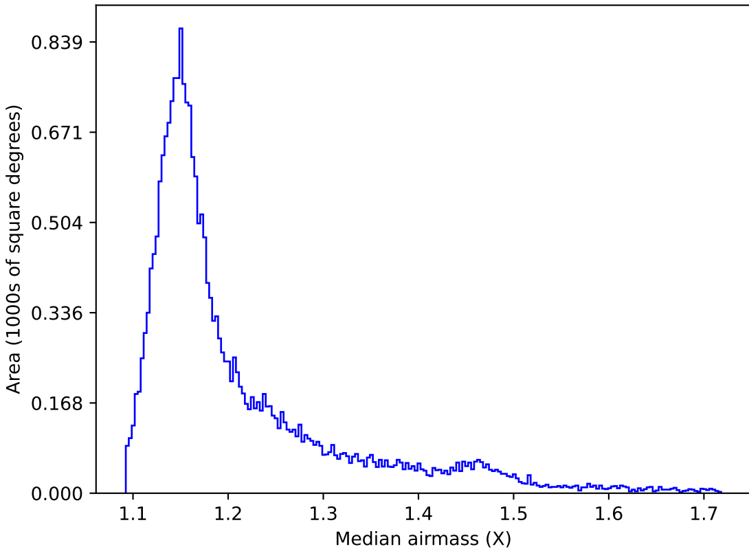
extra_ss_neo7_v3.4_10yrs All sky y band: Median airmass
