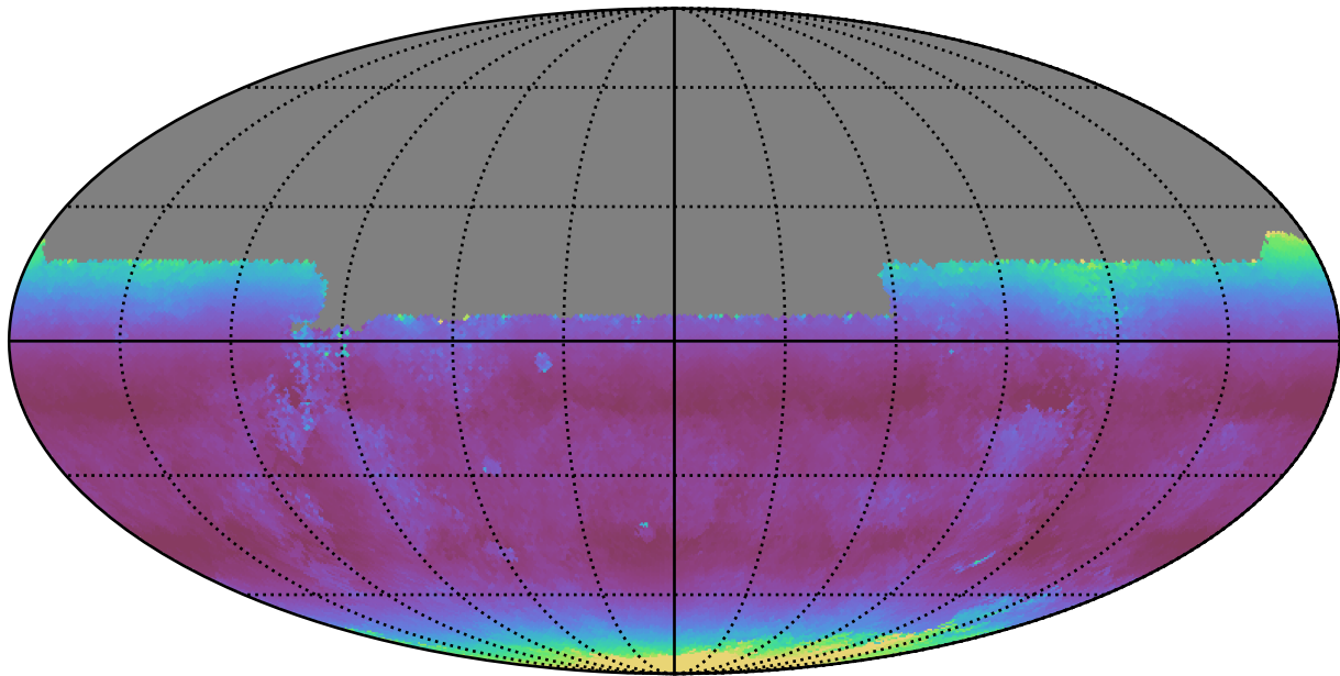
extra_ss_neo7_v3.4_10yrs All sky u band: Median airmass
