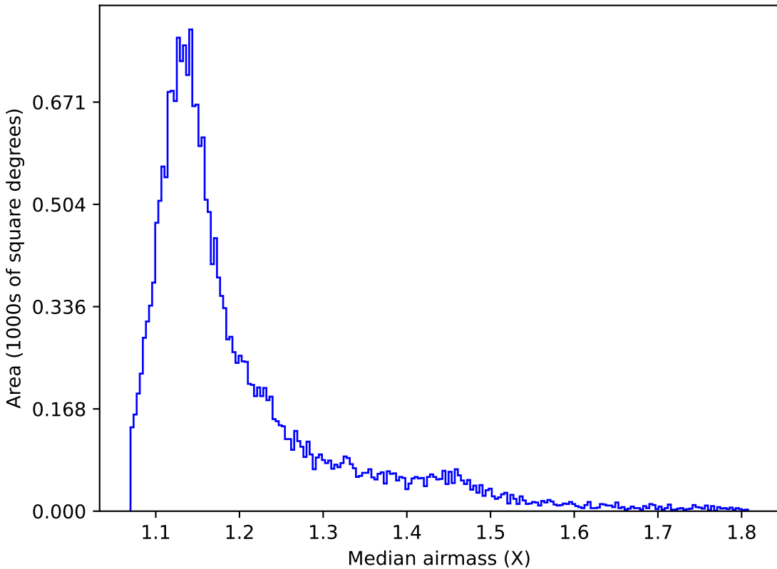
extra_ss_neo7_v3.4_10yrs All sky u band: Median airmass
