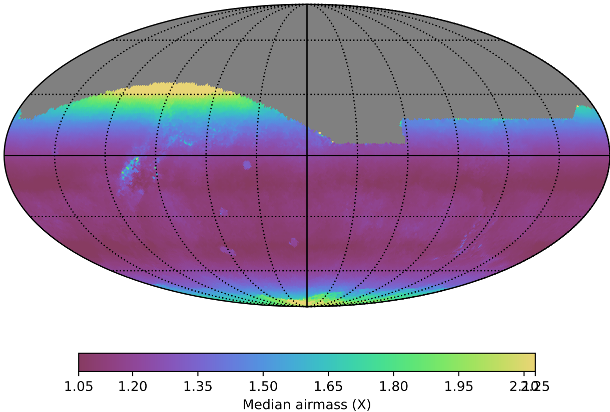
extra_ss_neo7_v3.4_10yrs All sky r band: Median airmass
