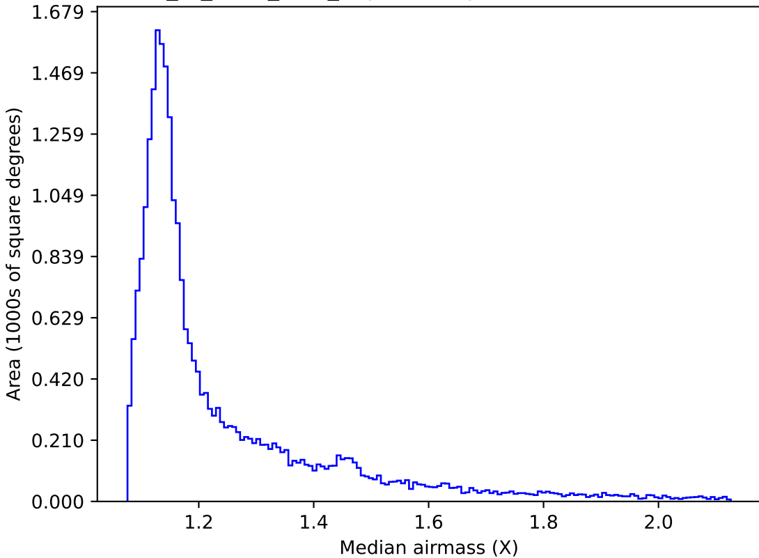
extra_ss_neo7_v3.4_10yrs All sky r band: Median airmass
