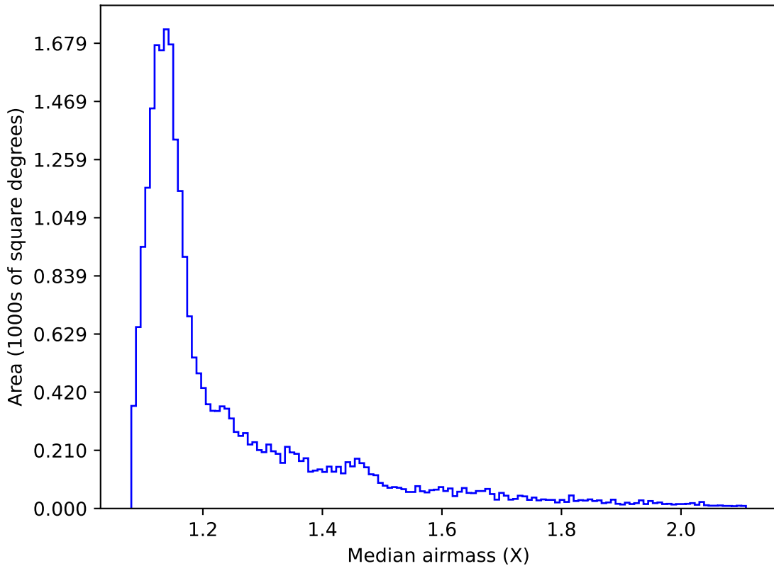
extra_ss_neo7_v3.4_10yrs All sky i band: Median airmass
